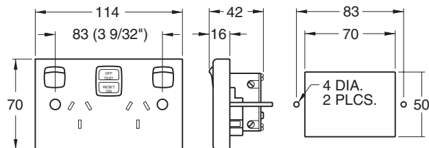
PANEL CUTOUT
